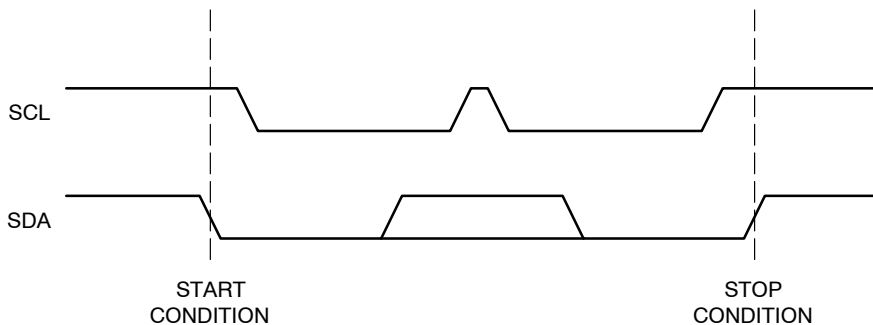
Figure 2. START/STOP Conditions
