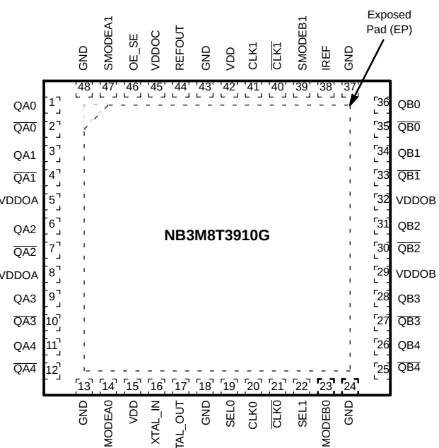
Figure 2. QFN-48 Pinout Configuration (Top View)
