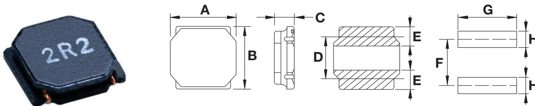
PCB Pattern
