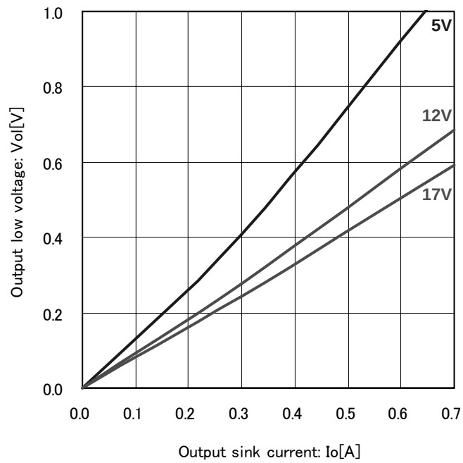
Fig.8 Output low voltage (T a =25°C)
