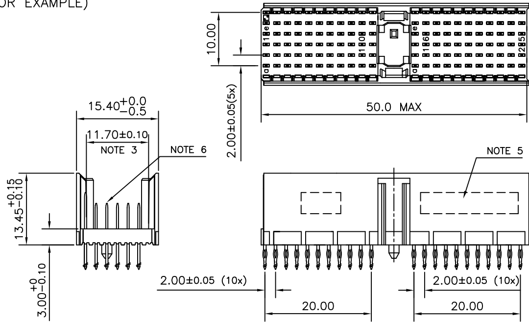
LOADED CONNECTOR ASSEMBLY (FOR EXAMPLE)
