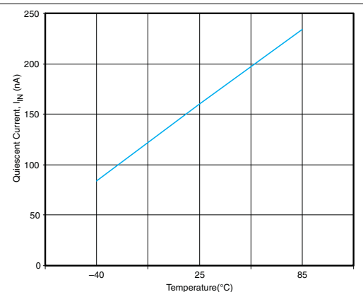
Figure 5. Quiescent Current vs Temperature ( V_{IN} = 3.3 V, I_{OUT} = 0 )
