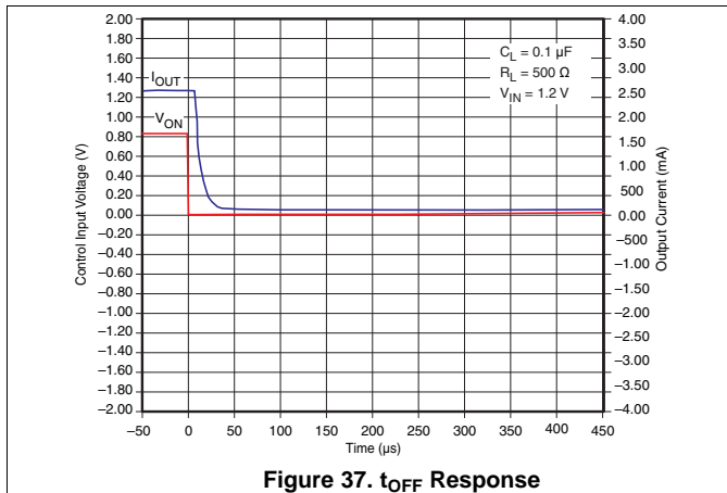
Figure 37. t_{OFF} Response
