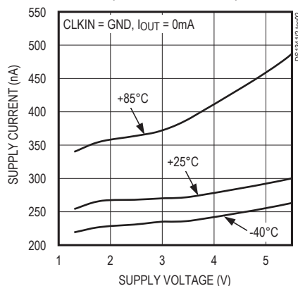
DS1342 I_{\text{CCT}} SUPPLY CURRENT vs. SUPPLY VOLTAGE (EGFIL = 1, DOSF = 0)
