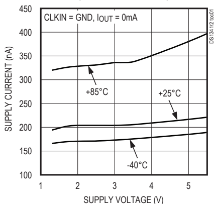
DS1342 I_{\text{CCT}} SUPPLY CURRENT vs. SUPPLY VOLTAGE (EGFIL = 0, DOSF = 1)
