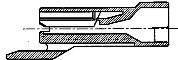
断面 "A" - "A" SECT.
