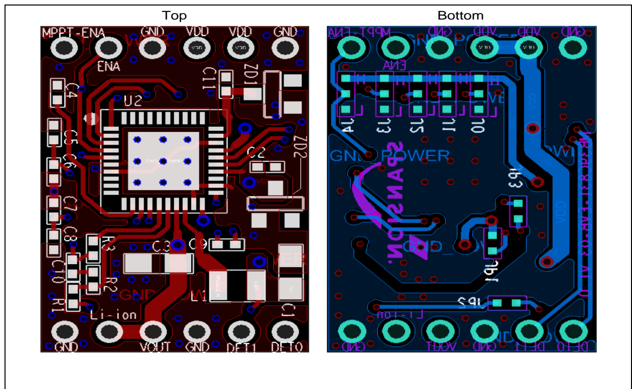
Figure 6. Layout
