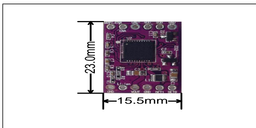
Figure 1. Board Size
