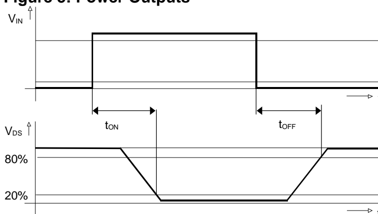
Figure 5: Power Outputs
