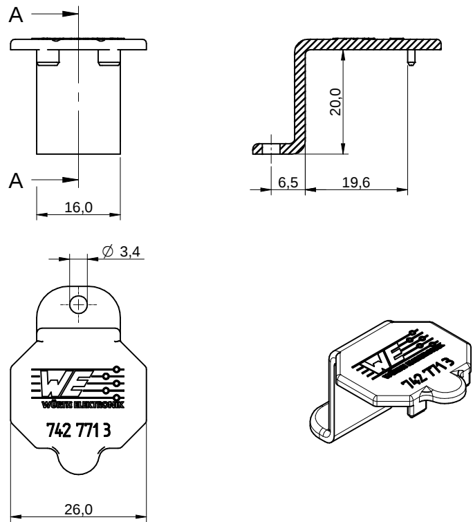
sectional drawing A-A
