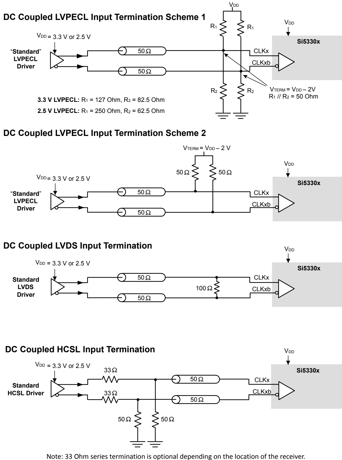
Figure 2.4. Differential DC-Coupled Input Terminations
