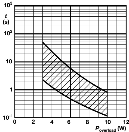
NFR25 This graph is based on measured data which may deviate according to the application. Fusing Characteristics: 15 \Omega \leq R \leq 15 k\Omega
