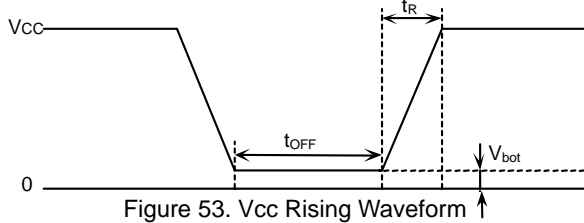
Figure 53. Vcc Rising Waveform
