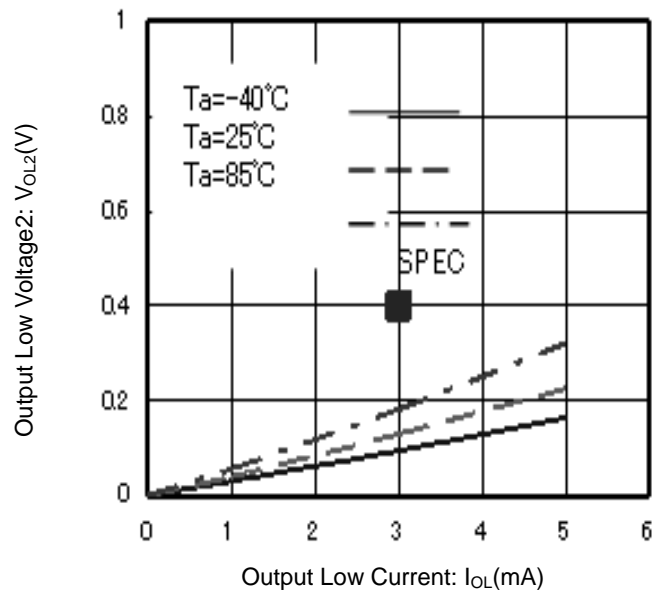
Figure 5. Output Low Voltage2 vs Output Low Current (V<sub>CC</sub>=1.7V)
