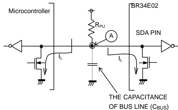
Figure 45. I/O Circuit
