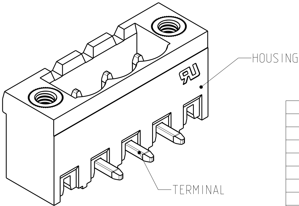
796864-3 AS SHOWN
