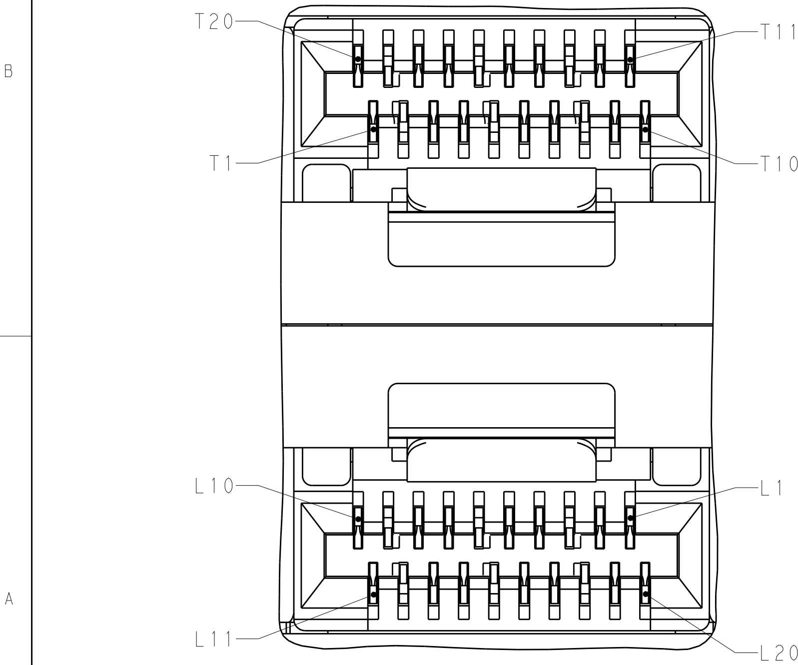
DETAIL A 2 PLACES SCALE 10:1
