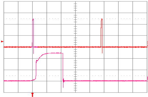
Fig. 2.5V.15: Load current (top trace, 20 A/div, 20 ms/div) into a 10 mΩ short circuit during restart, at V in = 48 V. Bottom trace (20 A/div, 1 ms/div) is an expansion of the on-time portion of the top trace.
