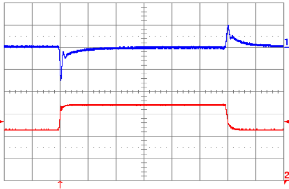
Fig. 2.0V.9: Output voltage response to load current step-change (22.5 A – 33.75 A – 22.5 A) at V_{in} = 48\text{ V} . Top trace: output voltage (20 mV/div.). Bottom trace: load current (10 A/div). Current slew rate: 1 A/ \mu\text{s} . C_o = 470\text{ }\mu\text{F} tantalum + 1 \mu\text{F} ceramic. Time scale: 0.2 ms/div.
