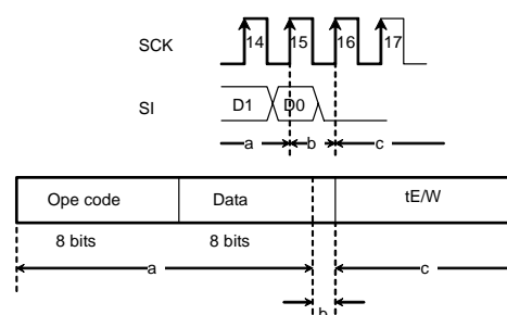
Figure 40. WRSR cancel valid timing
