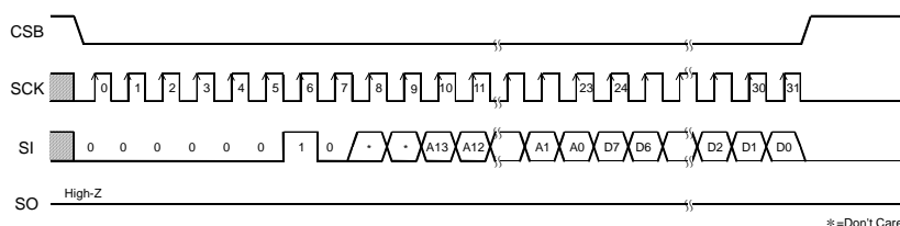
Figure 33. Write command
