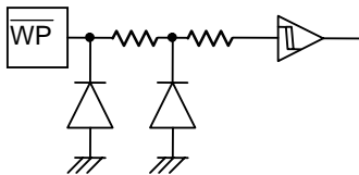
Figure 50. WP input equivalent circuit
