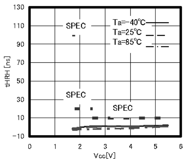
Figure 24. HOLD release hold time t_{HRH}
