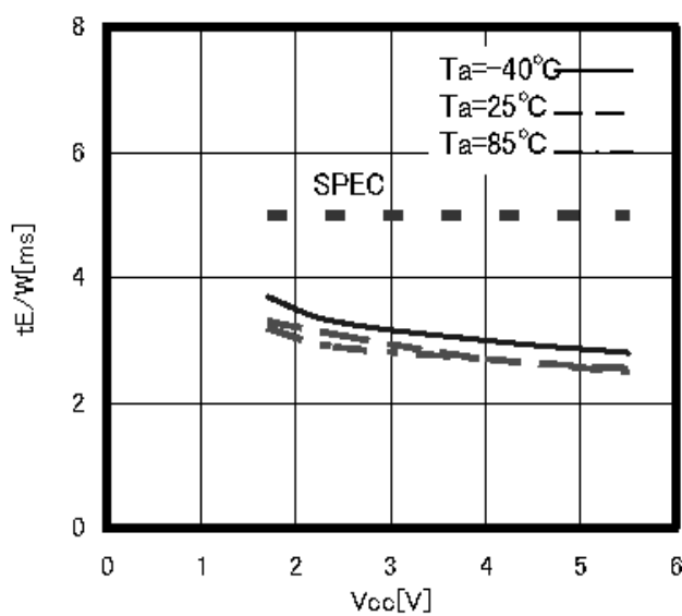
Figure 29. Write cycle time tE/W
