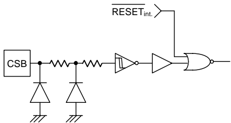
Figure 46. CSB input equivalent circuit
