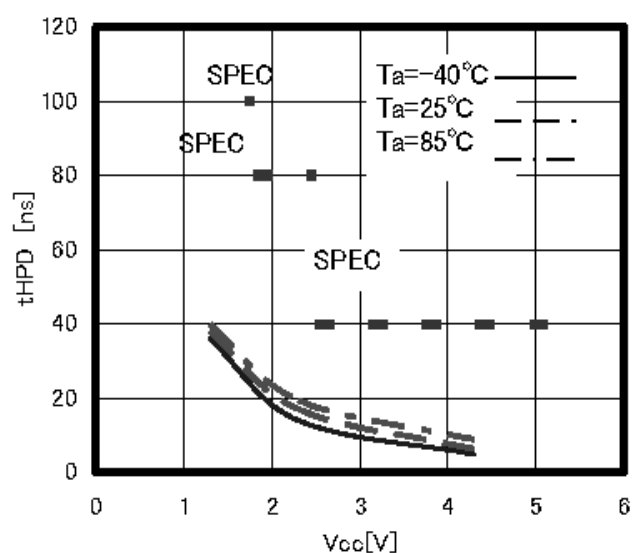
Figure 26. Time from HOLD to output change t_{HPD}
