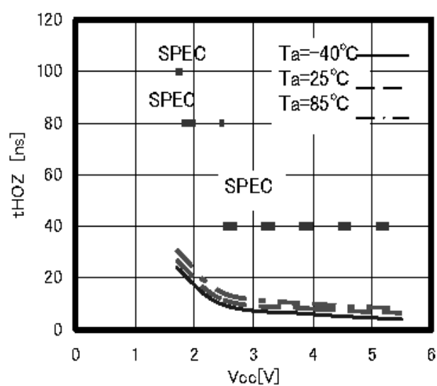
Figure 25. Time from HOLD to output High-Z t_{HOZ}
