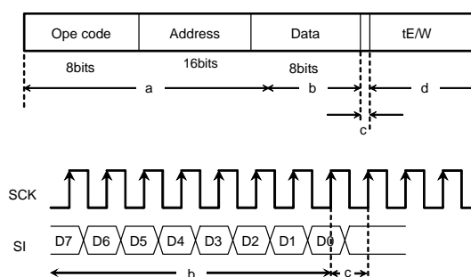
Figure 39. WRITE cancel valid timing
