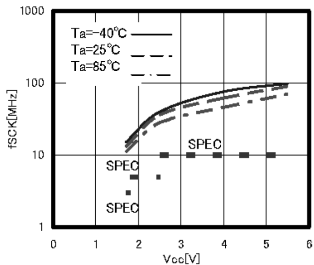
Figure 13. SCK frequency f_{SCK}
