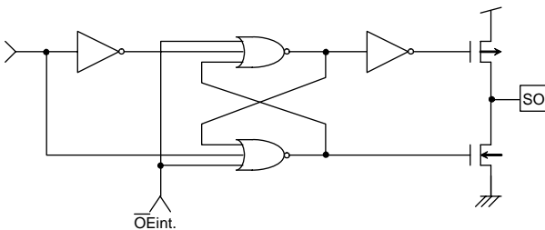
Figure 45. SO output equivalent circuit
