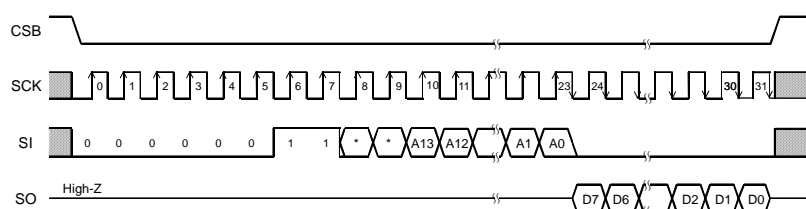
Figure 32. Read command
