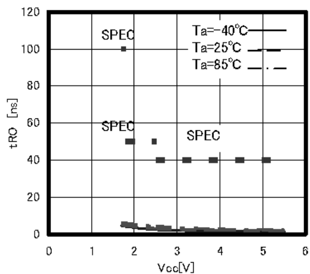
Figure 27. Output rise time t_{RO}
