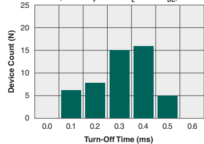
Typical Turn-Off Time (N=50, I_F=8mA , I_L=85mA_{DC} )
