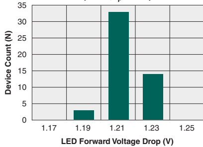
Typical LED Forward Voltage Drop (N=50, I_F=8mA )
