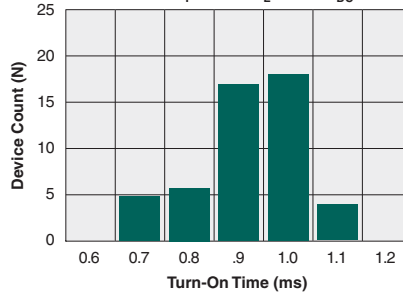
Typical Turn-On Time (N=50, I_F=8mA , I_L=85mA_{DC} )
