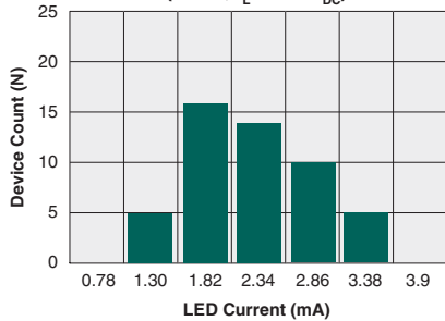
Typical I_F for Switch Operation (N=50, I_L=85mA_{DC} )
