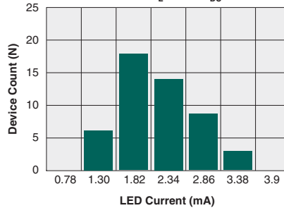
Typical I_F for Switch Dropout (N=50, I_L=85mA_{DC} )
