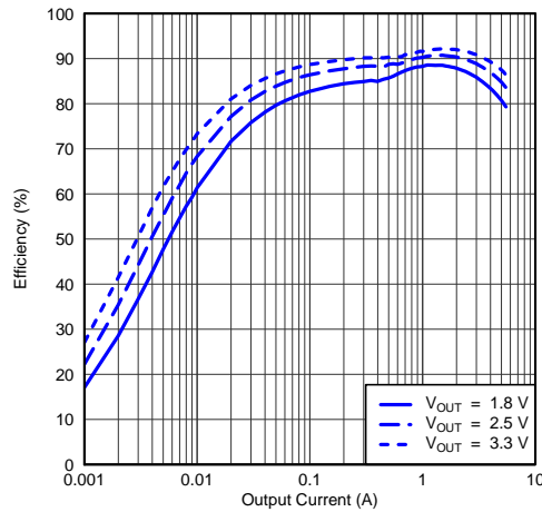
Figure 11. Light Load Efficiency vs Output Current
