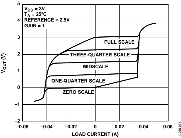
图33. 3 V时的源电流和吸电流能力(增益 = 1)
