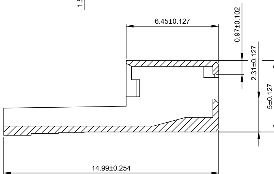
Section J-J
