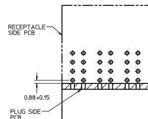
SECTION Z-Z
