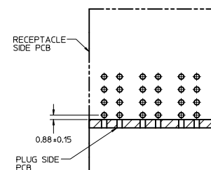
SECTION Z-Z
