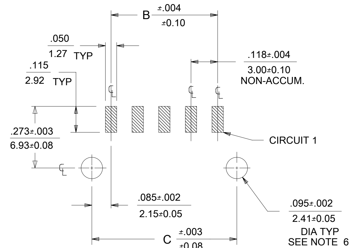
PCB LAYOUT: COMPONENT SIDE RECOMMENDED PCB THICKNESS: .062/1.57
