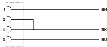
Circuit diagram
