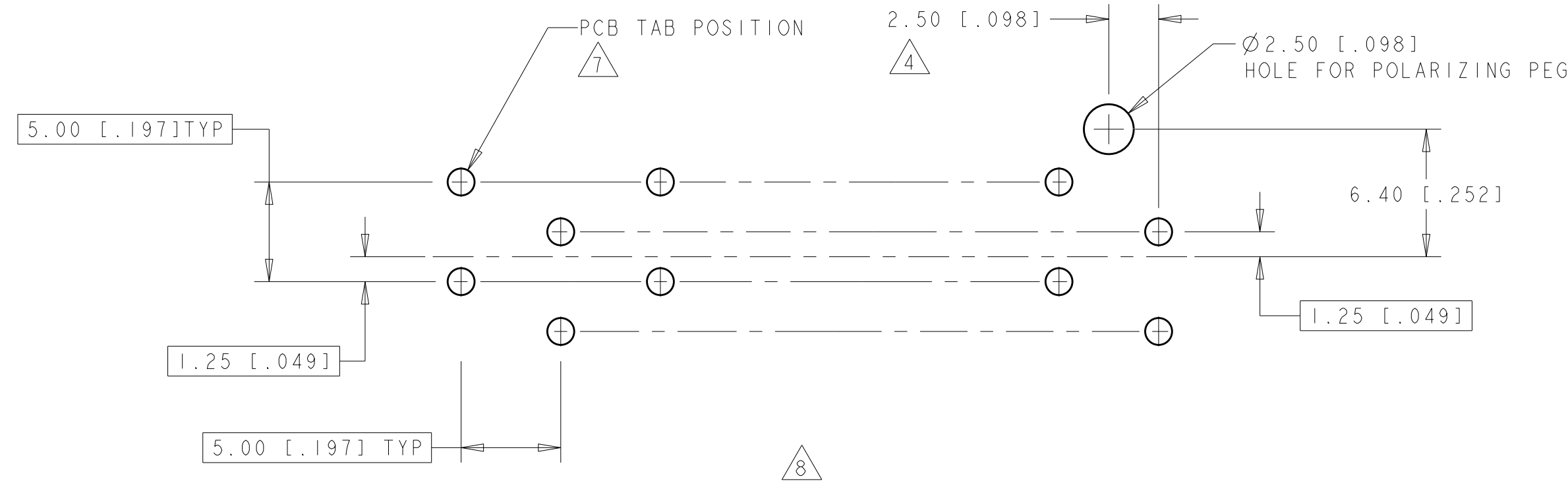
PCB LAYOUT - COMPONENT SIDE PCB 1.5 \pm 0.2 [ .059 \pm .007 ] THICK SCALE 4:1
