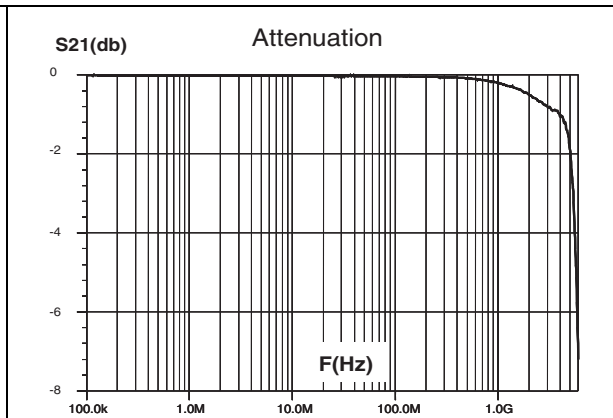
Figure 4. Frequency response
