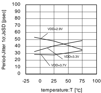
Fig.47 36MHz Period-Jitter 1σ: JsSD temperature characteristic s
