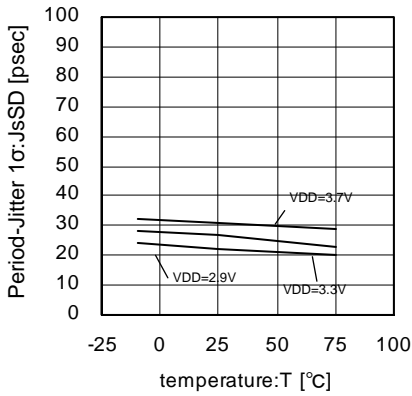
Fig.42 27MHz Period-Jitter 1σ: JsSD temperature characteristics
