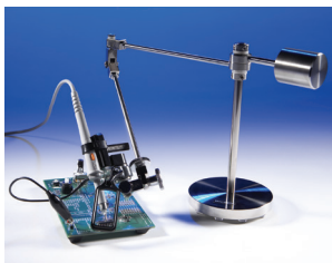
N2784A one-arm probe positioner
