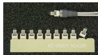
N5425B/26A high bandwidth ZIF solder-in probe head and tips for InfiniiMax probes
