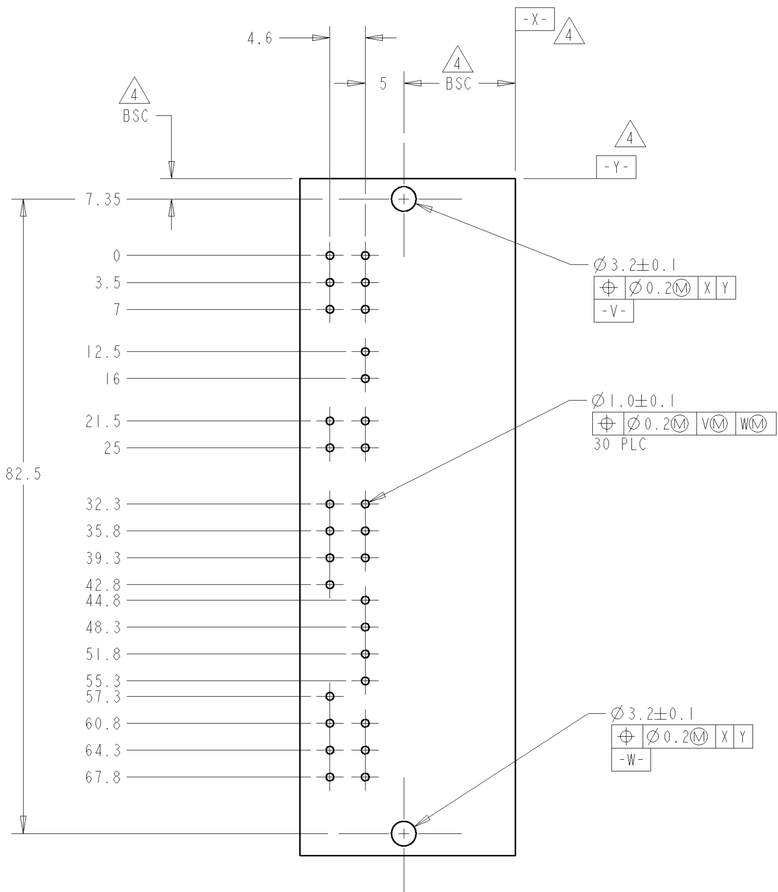
P.C. BOARD LAYOUT RECOMMENDED BOARD THICKNESS 1.60 ± 0.15mm TOLERANCES ± 0.1
