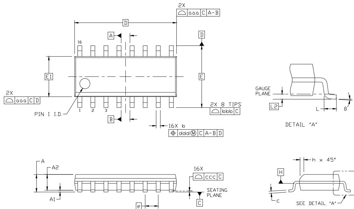
Figure 3. 16-Pin SOIC
