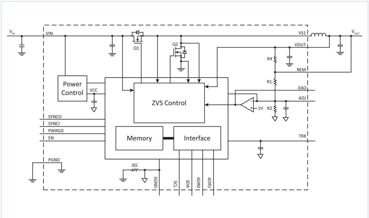
Simplified block diagram ( I 2C™ pins SCL, SDA, ADR0, and ADR1 only active for PI33xx-20 device versions)
