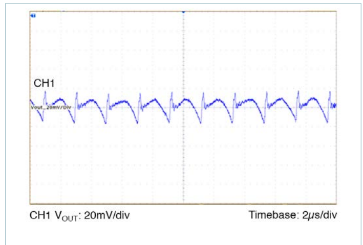
Figure 11 — Output ripple 24V IN , 1.8V OUT at 10A
