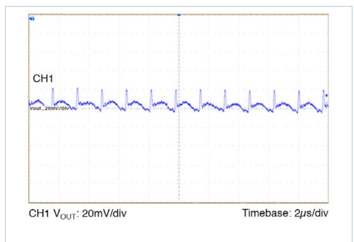
Figure 12 — Output ripple 24V IN , 1.8V OUT at 5A
