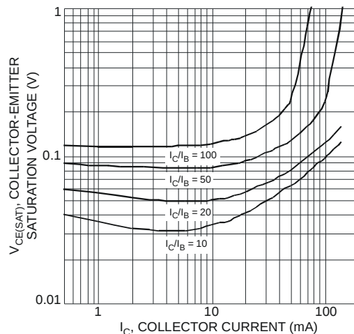
Fig. 7 Typical Collector-Emitter Saturation Voltage vs. Collector Current
