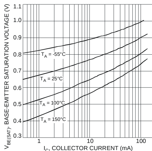
Fig. 9 Typical Base-Emitter Saturation Voltage vs. Collector Current
