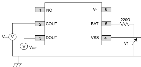
Figure 20. Test Circuit 1
