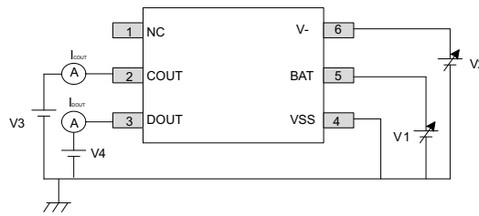
Figure 23. Test Circuit 4
