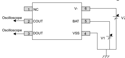
Figure 24. Test Circuit 5
