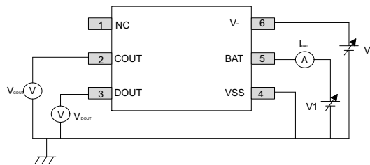
Figure 21. Test Circuit 2
