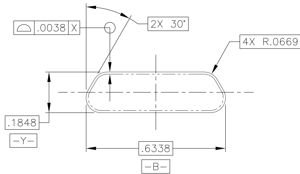
INTERFACE DETAIL
