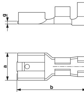
Dimensional drawing
