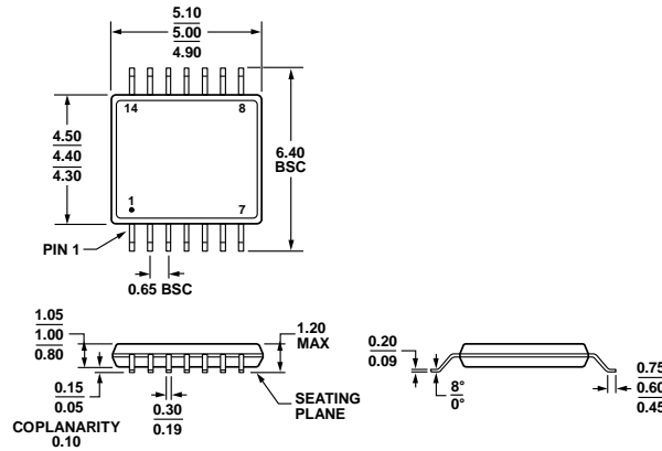
COMPLIANT TO JEDEC STANDARDS MO-153-AB-1 Figure 53. 14-Lead Thin Shrink Small Outline Package [TSSOP] (RU-14) Dimensions shown in millimeters
