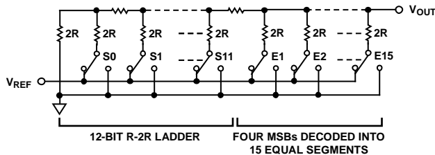
Figure 40. DAC Ladder Structure
