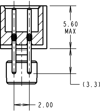
SECTION Y-Y
