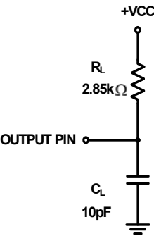
FIGURE 4. EQUIVALENT LOAD CIRCUIT
