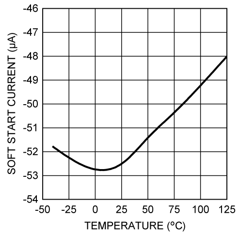
Figure 8. Soft-Start Current vs Temperature
