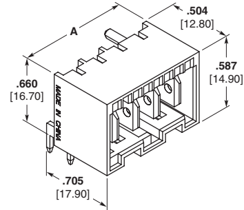
Right-Angle Orientation
