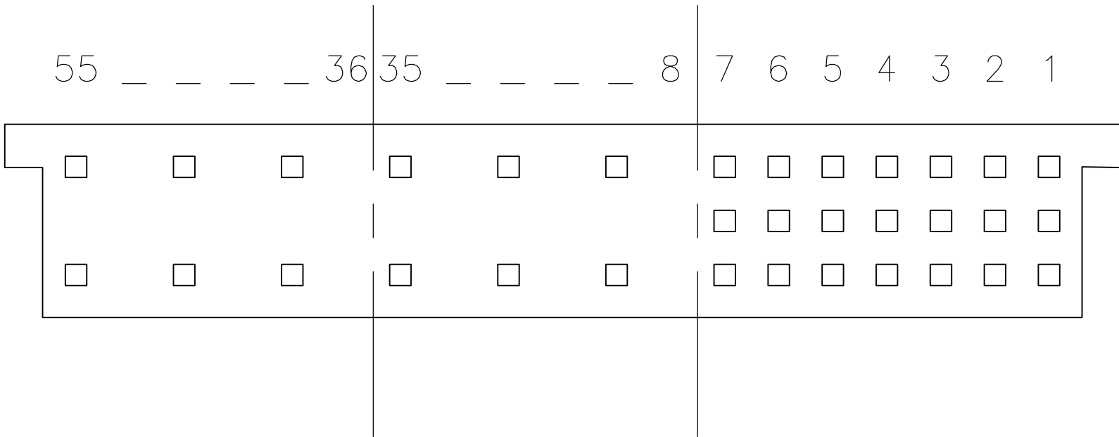
CONTACT LOADING PATTERN 69 CONTACTS P/N 532834-2
