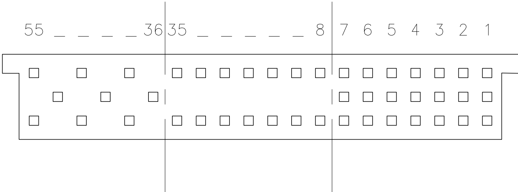
CONTACT LOADING PATTERN 107 CONTACTS P/N 532834-1
