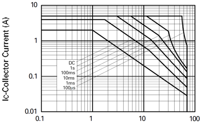
Safe Operating Area
