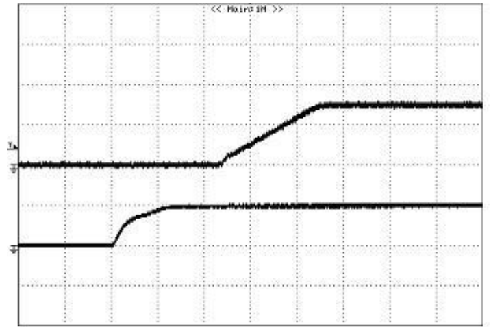
Figure 16: Turn on delay time at 5Vin, 1.5V/3A out Top: Vout, 1V/div, Bottom: Vin, 5V/div; 2mS/div
