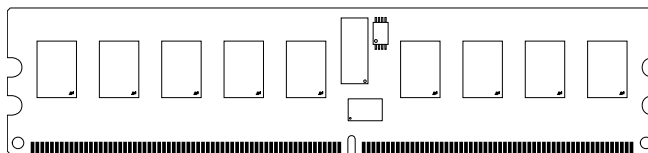
Figure 1: 240-Pin RDIMM (MO-237 R/C G)
