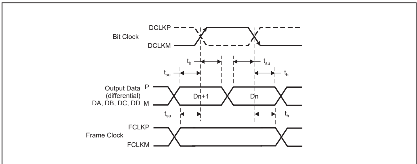
Figure 2. LVDS Timings
