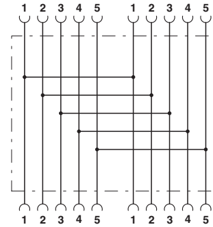
Circuit diagram
