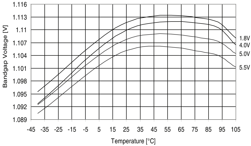
Figure 32-279. ATmega3290A: Bandgap Voltage vs. Temperature
