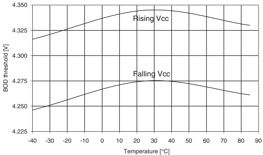
Figure 31-344. Atmel ATmega3290PA: BOD Thresholds vs. temperature (BOD level is 4.3V).
