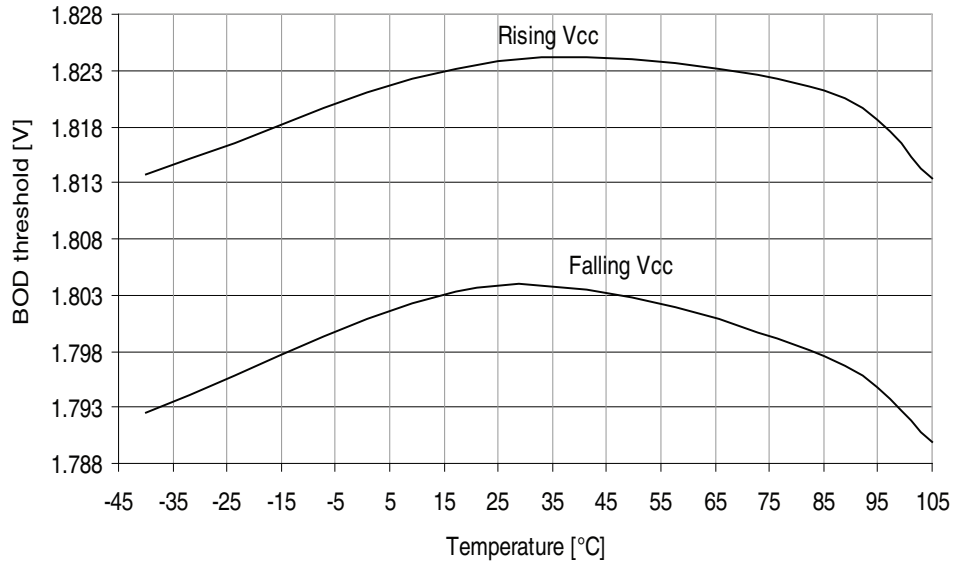
Figure 32-277. ATmega3290A - 105°C: BOD Thresholds vs. Temperature (BOD Level is 1.8V)
