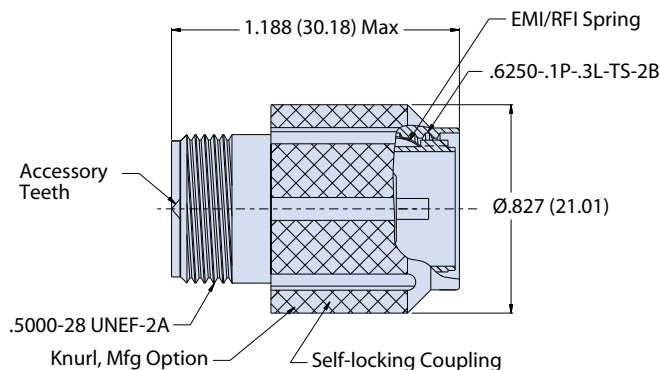
805-088 Plug Adapter with Accessory Thread
