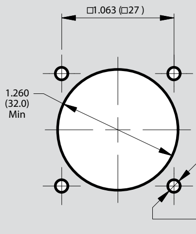
SQUARE FLANGE REAR MOUNT RECOMMENDED MOUNTING HOLES
