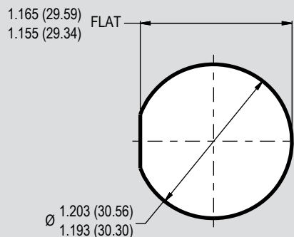
JAM NUT RECEPTACLE REAR PANEL MOUNT MAX PANEL THICKNESS .188 (4.78) MAX
