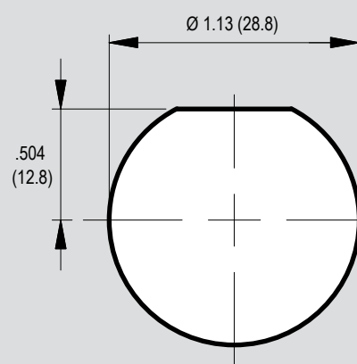
JAM NUT MOUNT RECOMMENDED MOUNTING HOLE PANEL THICKNESS .063-.126 (1.6 -3.2)
