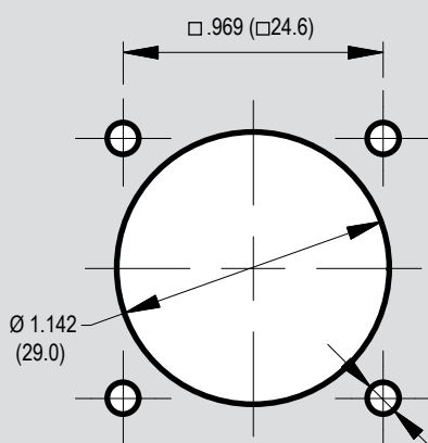
SQUARE FLANGE REAR MOUNT RECOMMENDED MOUNTING HOLES
