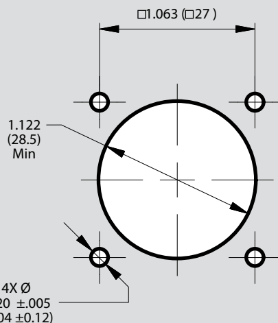
SQUARE FLANGE FRONT MOUNT RECOMMENDED MOUNTING HOLES
