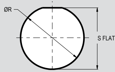
REAR PANEL MOUNT JAM NUT RECEPTACLE MAX PANEL THICKNESS .188 (4.78)
