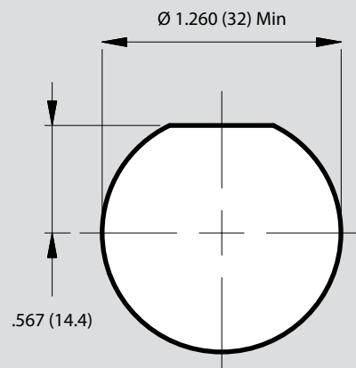
JAM NUT MOUNT RECOMMENDED MOUNTING HOLE PANEL THICKNESS .063-.126 (1.6 -3.2)
