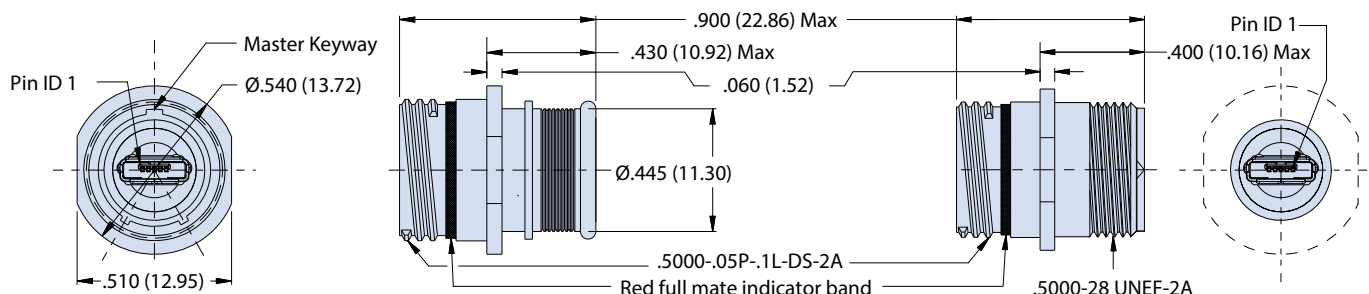
805-089-01 Receptacle with Shield Termination Porch
