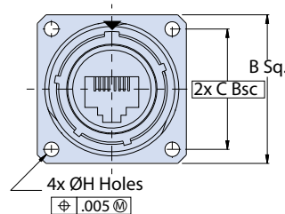
D0 - Wall Mount Receptacle With Round Holes (Mating Face)
