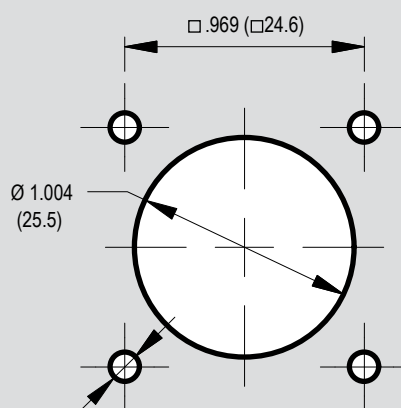
SQUARE FLANGE FRONT MOUNT RECOMMENDED MOUNTING HOLES
