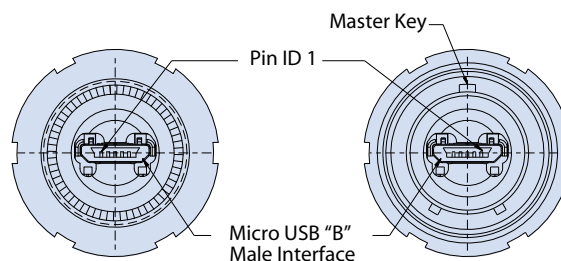
Face view of plug adapter as viewed from cable end.
