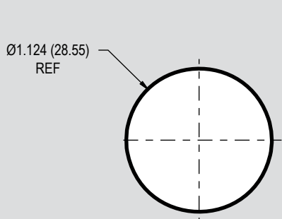
WALL MOUNT RECEPTACLE MAX PANEL THICKNESS .188 (4.78)
