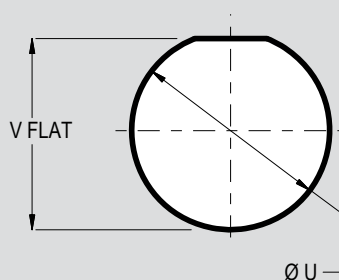
REAR PANEL MOUNT JAM NUT RECEPTACLE
