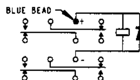
TERMINAL VIEW
